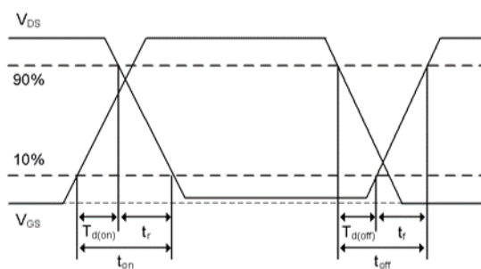
Fig17-2. Switching time waveform
