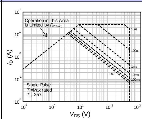
Fig.14 Safe operating area - Maximum
