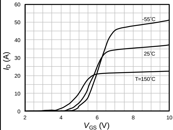
Fig.5 Transfer characteristics
